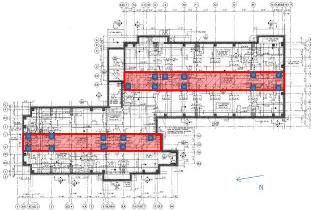
Figure 2: Foundation Trench
