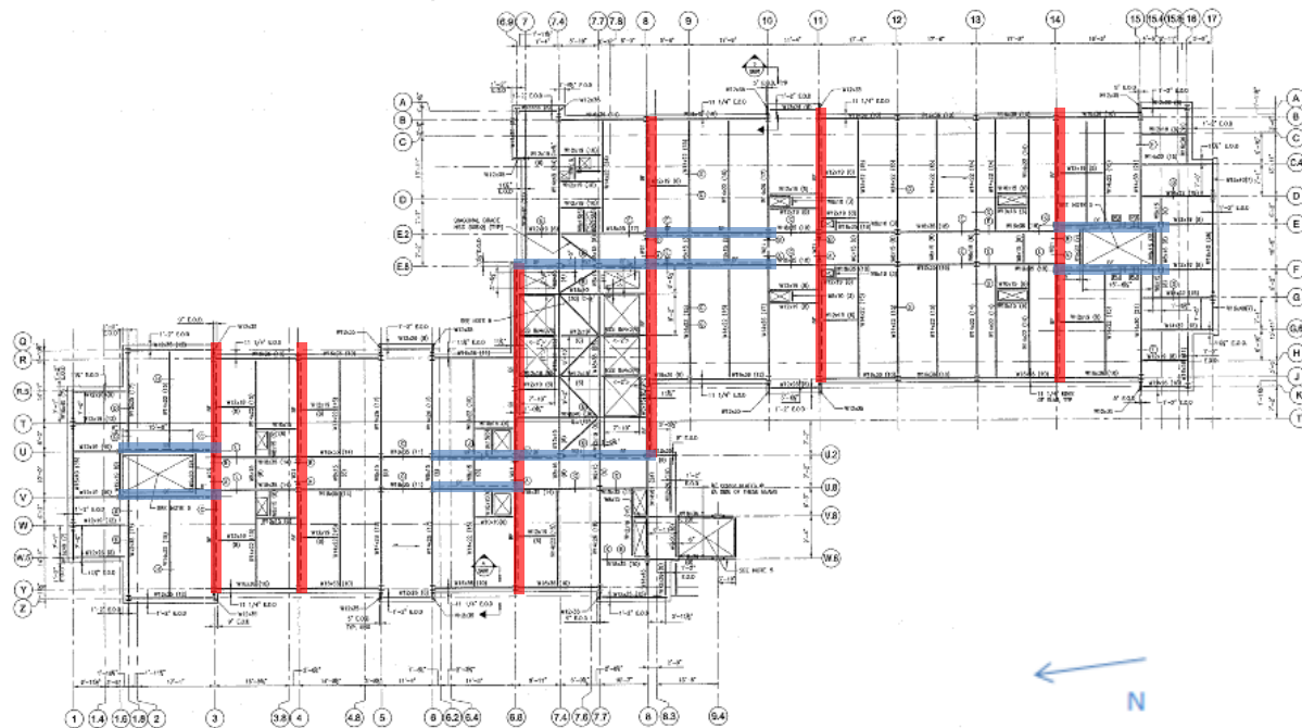
Figure 5: Typical plan with braced frame locations highlighted
